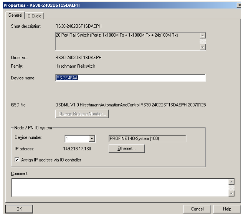
Figure 8: Dialog for entering the object name (= name of the Switch) and the IP parameter
